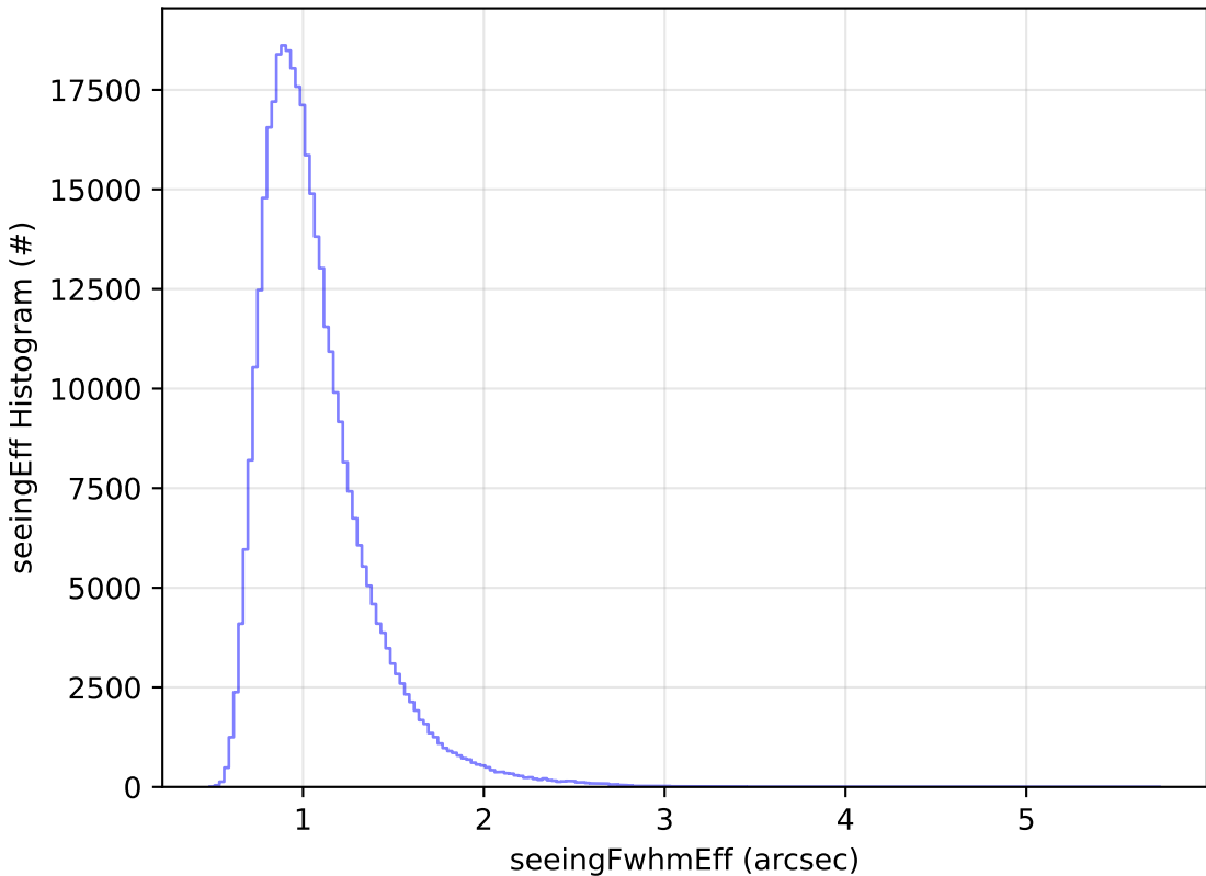
too_elab_r8_d2_giz_v3.4_10yrs WFD y band: seeingEff Histogram
