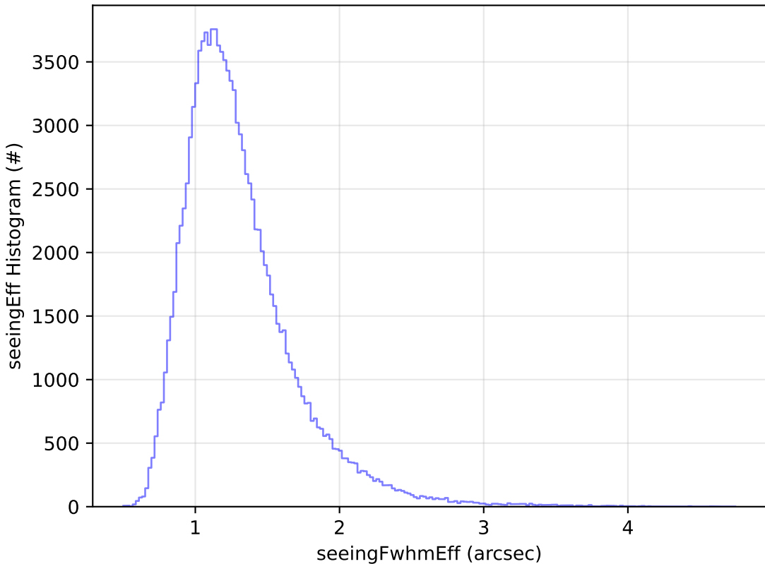
too_elab_r8_d2_giz_v3.4_10yrs WFD u band: seeingEff Histogram
