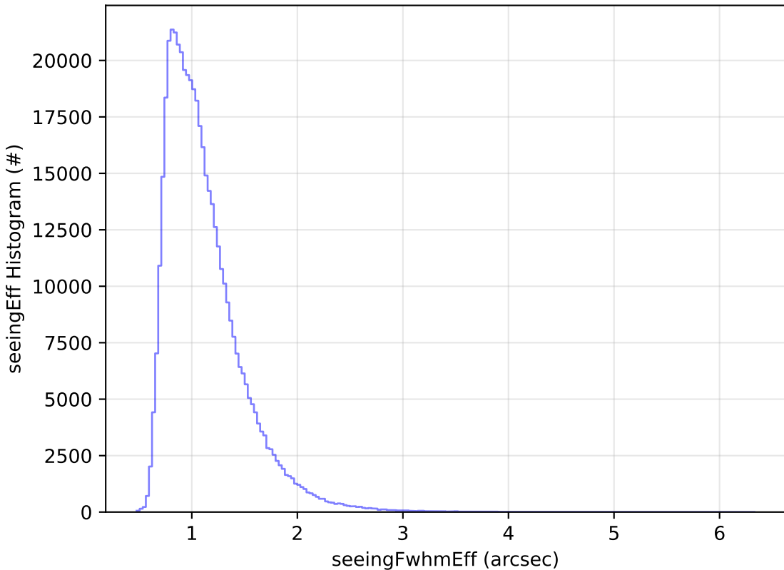
too_elab_r8_d2_giz_v3.4_10yrs WFD r band: seeingEff Histogram
