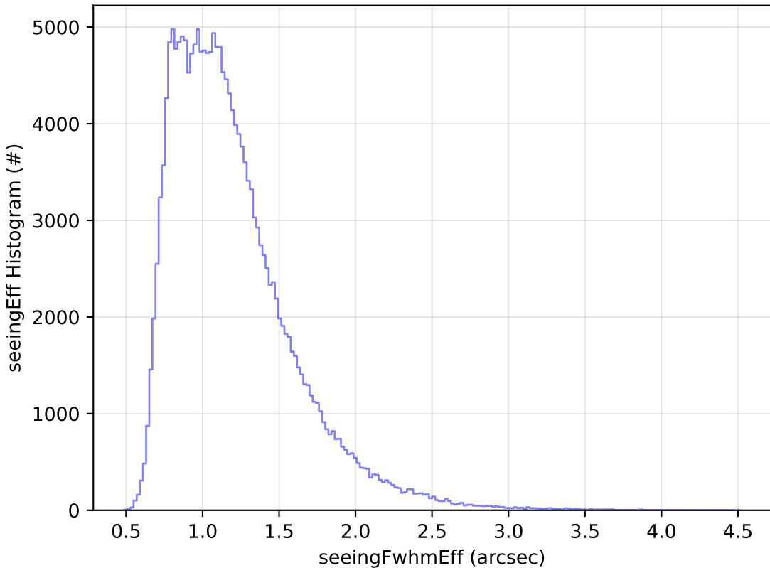
too_elab_r8_d2_giz_v3.4_10yrs WFD g band: seeingEff Histogram
