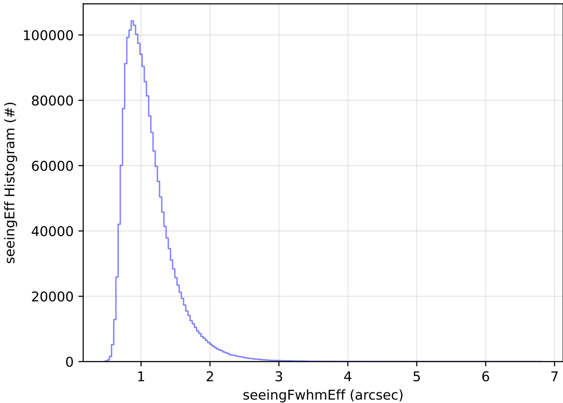
too_elab_r8_d2_giz_v3.4_10yrs WFD all bands: seeingEff Histogram
