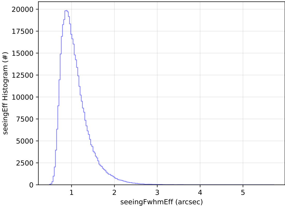
too_elab_r8_d2_giz_v3.4_10yrs All sky z band: seeingEff Histogram
