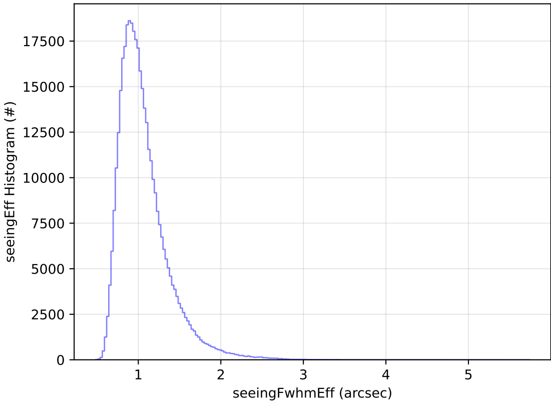
too_elab_r8_d2_giz_v3.4_10yrs All sky y band: seeingEff Histogram
