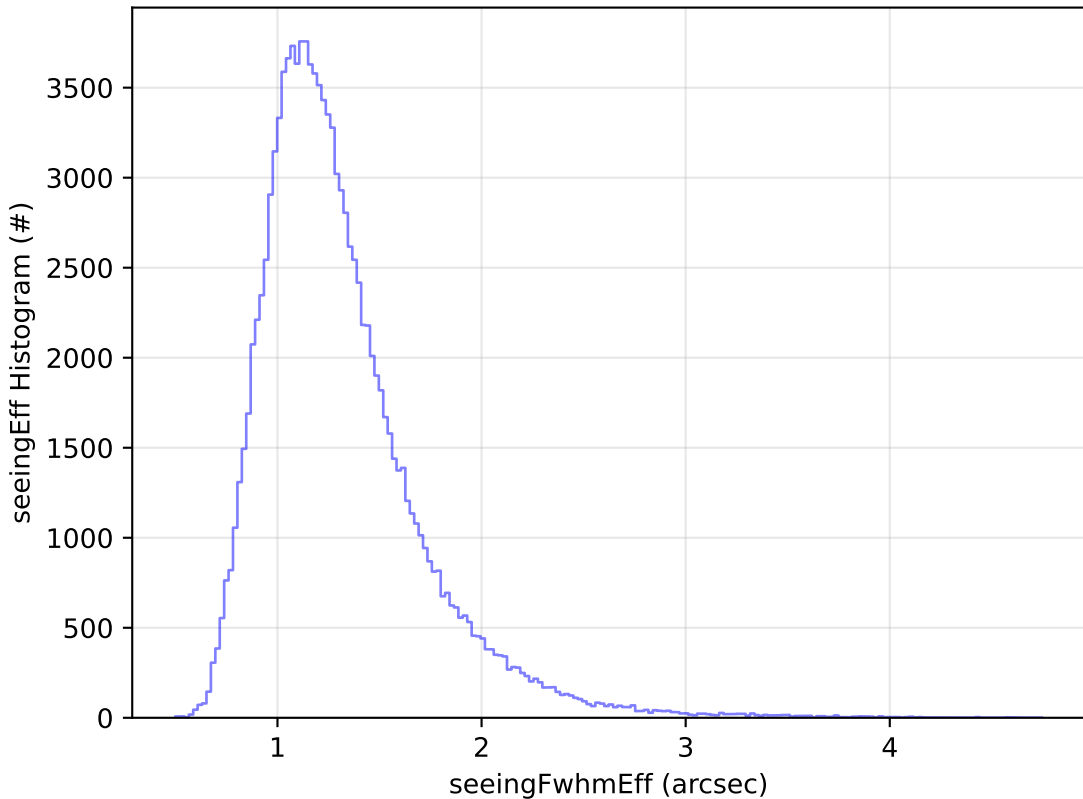
too_elab_r8_d2_giz_v3.4_10yrs All sky u band: seeingEff Histogram
