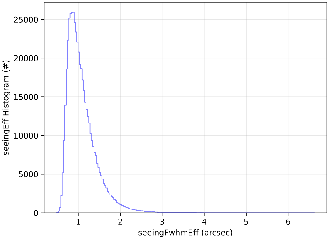
too_elab_r8_d2_giz_v3.4_10yrs All sky i band: seeingEff Histogram
