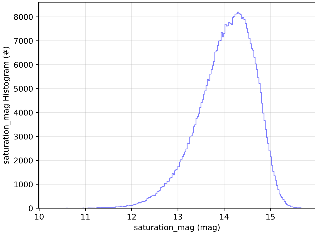
too_elab_r8_d2_giz_v3.4_10yrs WFD z band: saturation_mag Histogram
