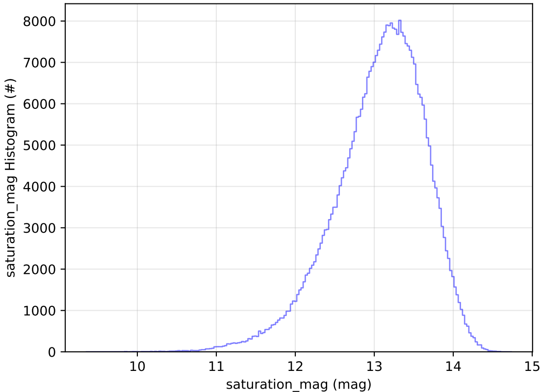
too_elab_r8_d2_giz_v3.4_10yrs WFD y band: saturation_mag Histogram
