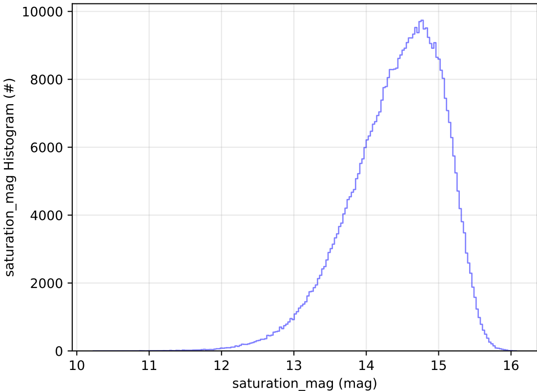
too_elab_r8_d2_giz_v3.4_10yrs WFD i band: saturation_mag Histogram
