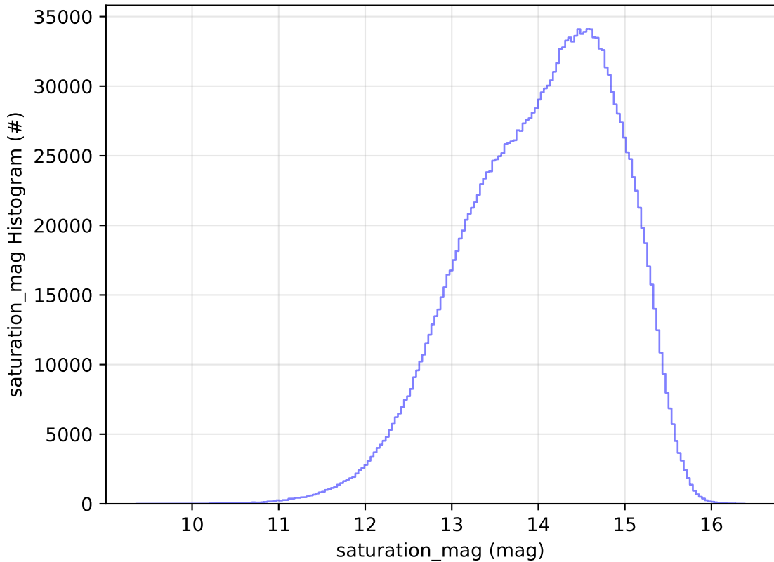
too_elab_r8_d2_giz_v3.4_10yrs WFD all bands: saturation_mag Histogram
