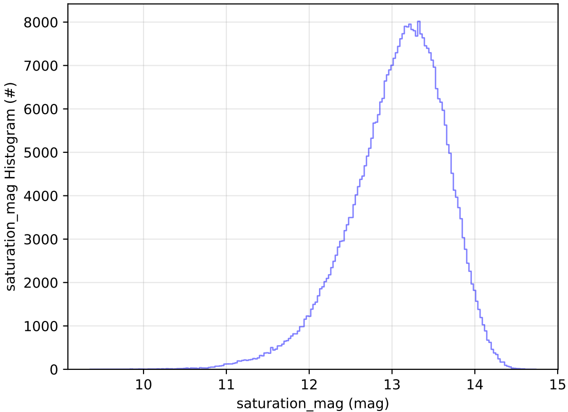
too_elab_r8_d2_giz_v3.4_10yrs All sky y band: saturation_mag Histogram
