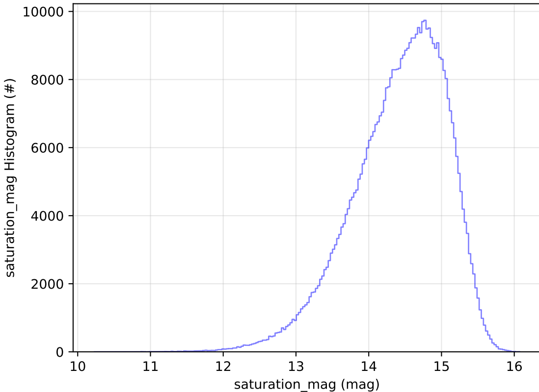
too_elab_r8_d2_giz_v3.4_10yrs All sky i band: saturation_mag Histogram
