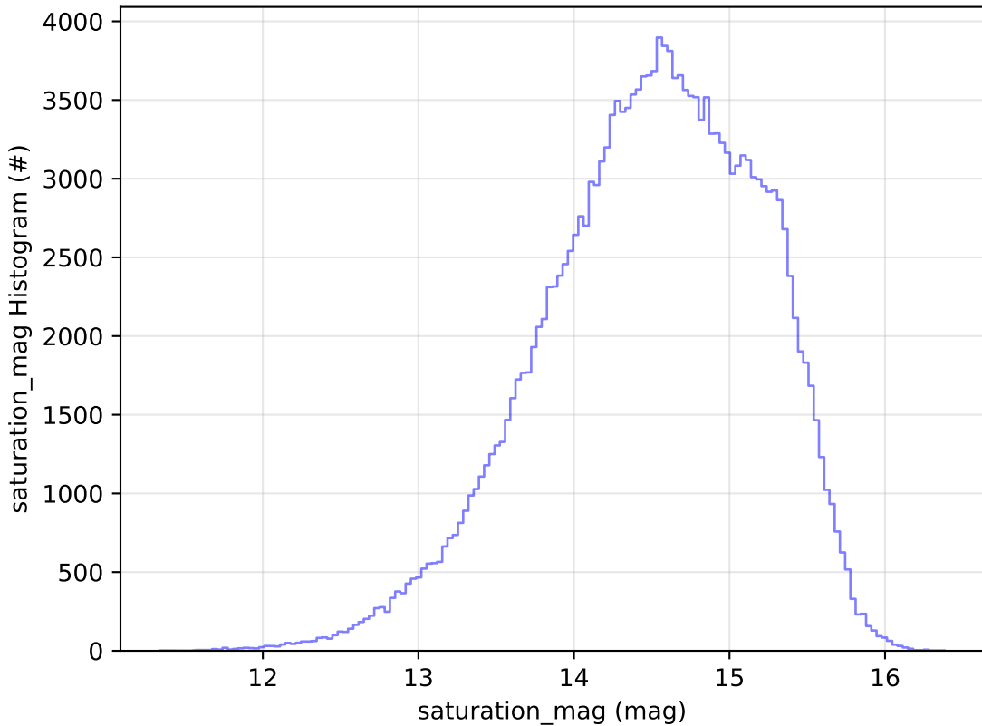
too_elab_r8_d2_giz_v3.4_10yrs All sky g band: saturation_mag Histogram
