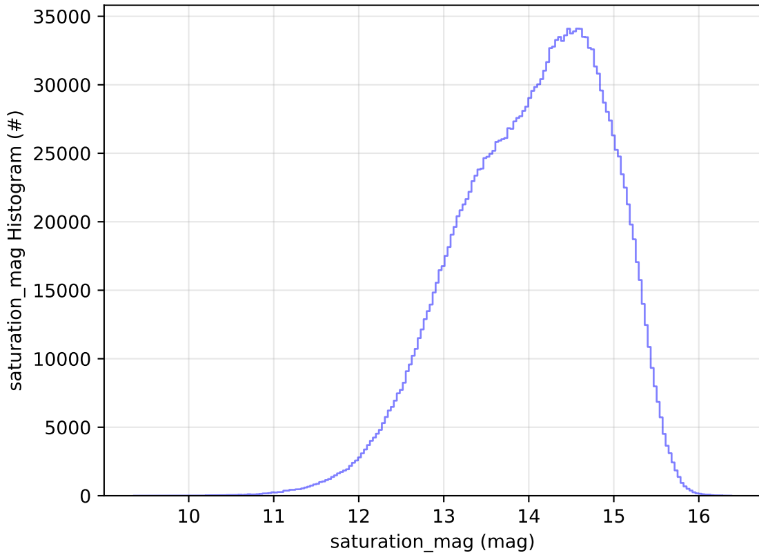
too_elab_r8_d2_giz_v3.4_10yrs All sky all bands: saturation_mag Histogram
