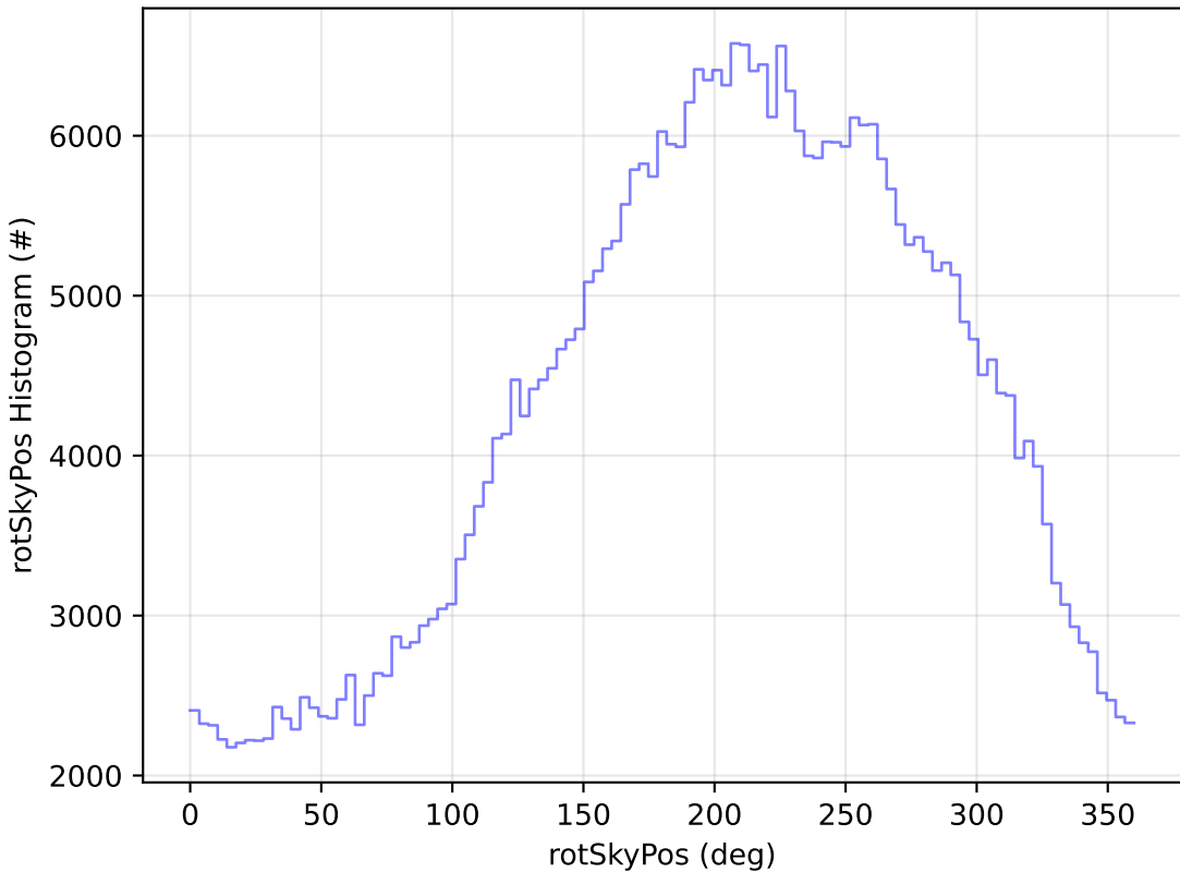
too_elab_r8_d2_giz_v3.4_10yrs WFD z band: rotSkyPos Histogram
