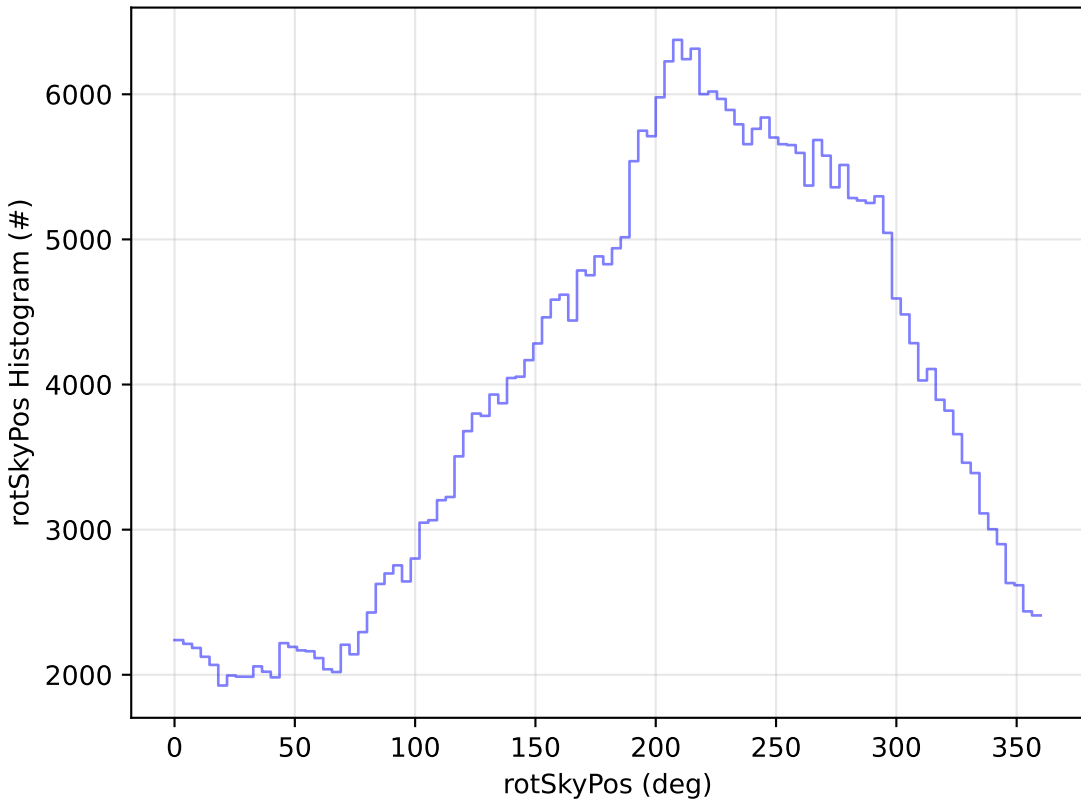
too_elab_r8_d2_giz_v3.4_10yrs WFD y band: rotSkyPos Histogram
