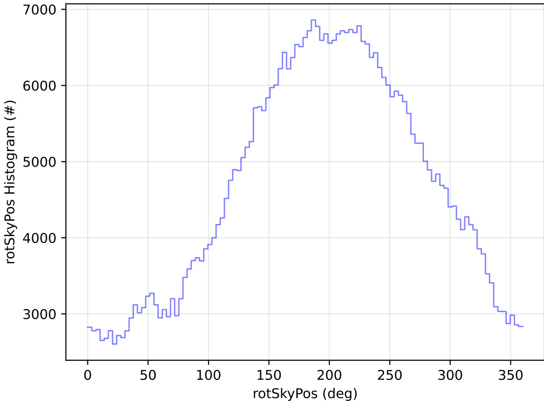
too_elab_r8_d2_giz_v3.4_10yrs WFD r band: rotSkyPos Histogram
