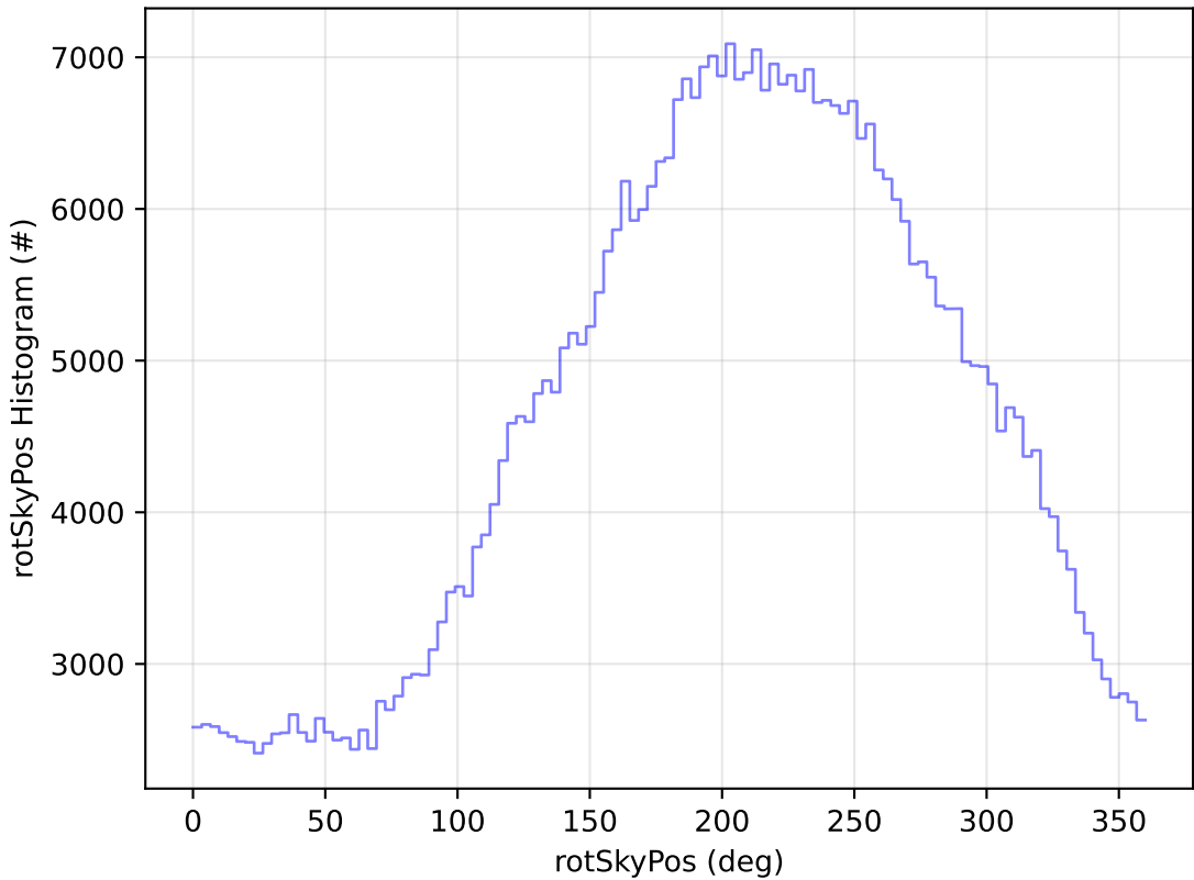
too_elab_r8_d2_giz_v3.4_10yrs WFD i band: rotSkyPos Histogram
