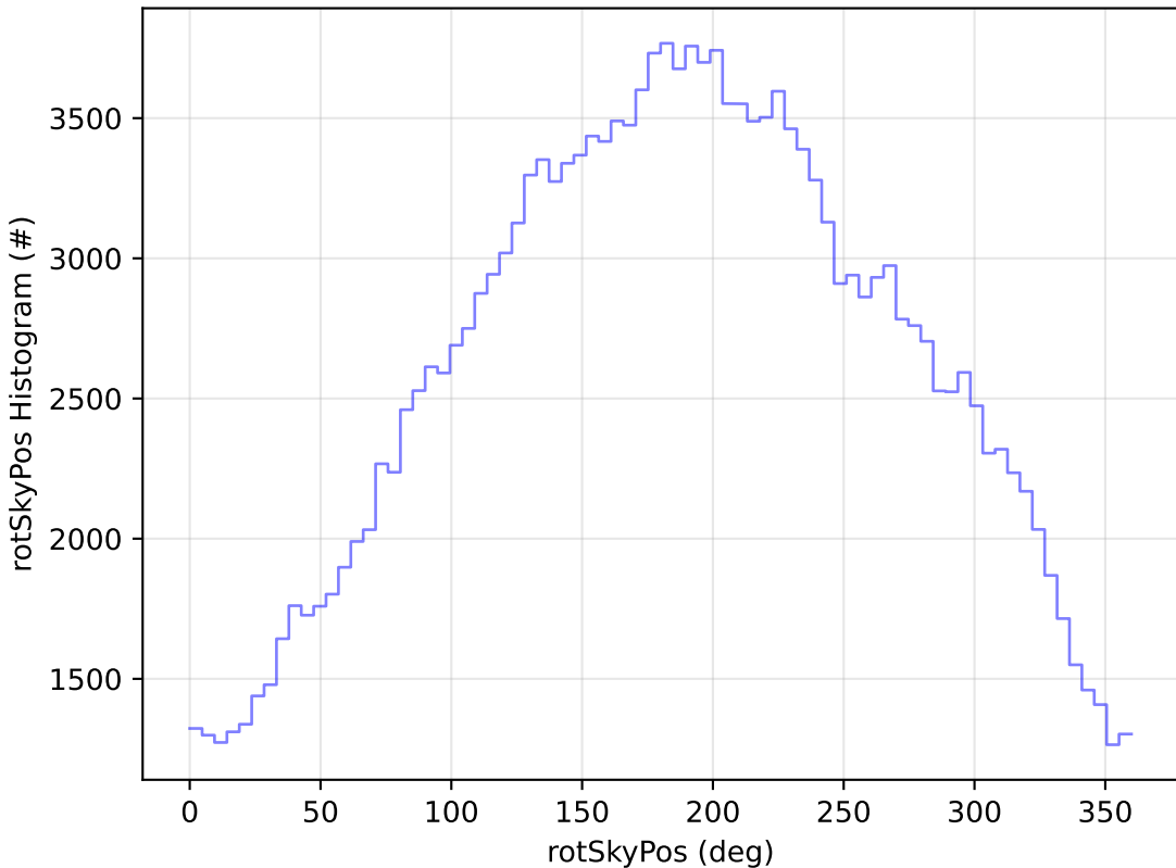
too_elab_r8_d2_giz_v3.4_10yrs WFD g band: rotSkyPos Histogram
