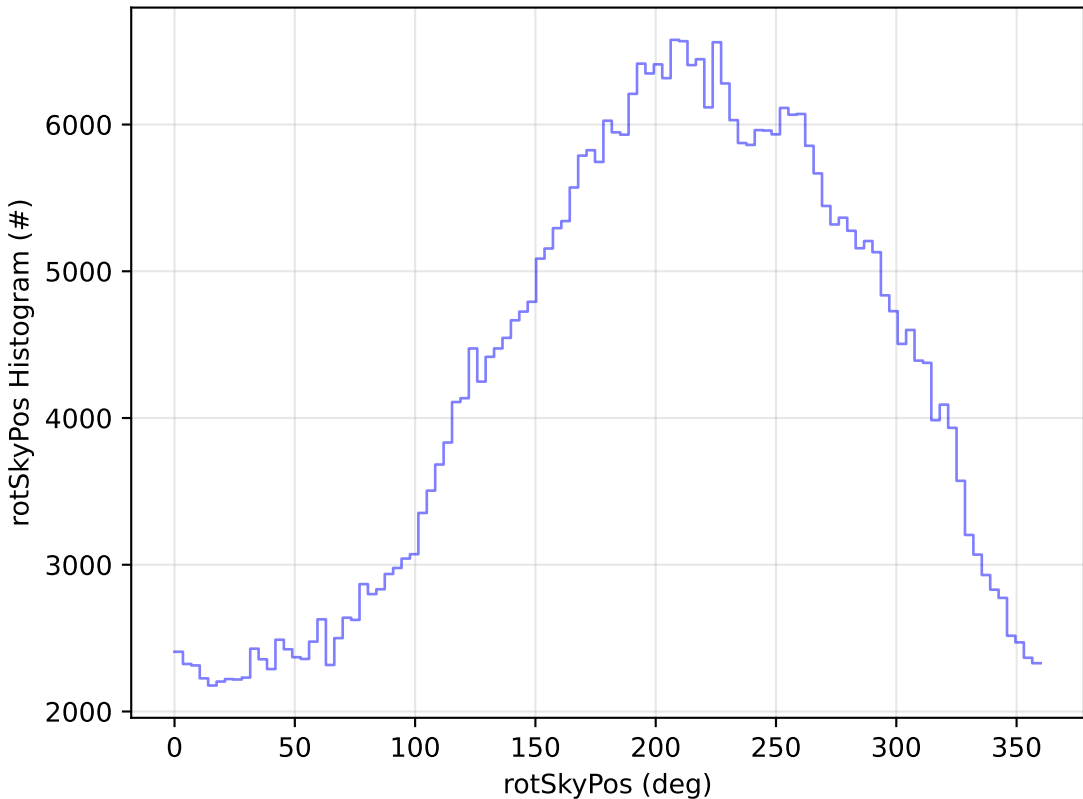
too_elab_r8_d2_giz_v3.4_10yrs All sky z band: rotSkyPos Histogram
