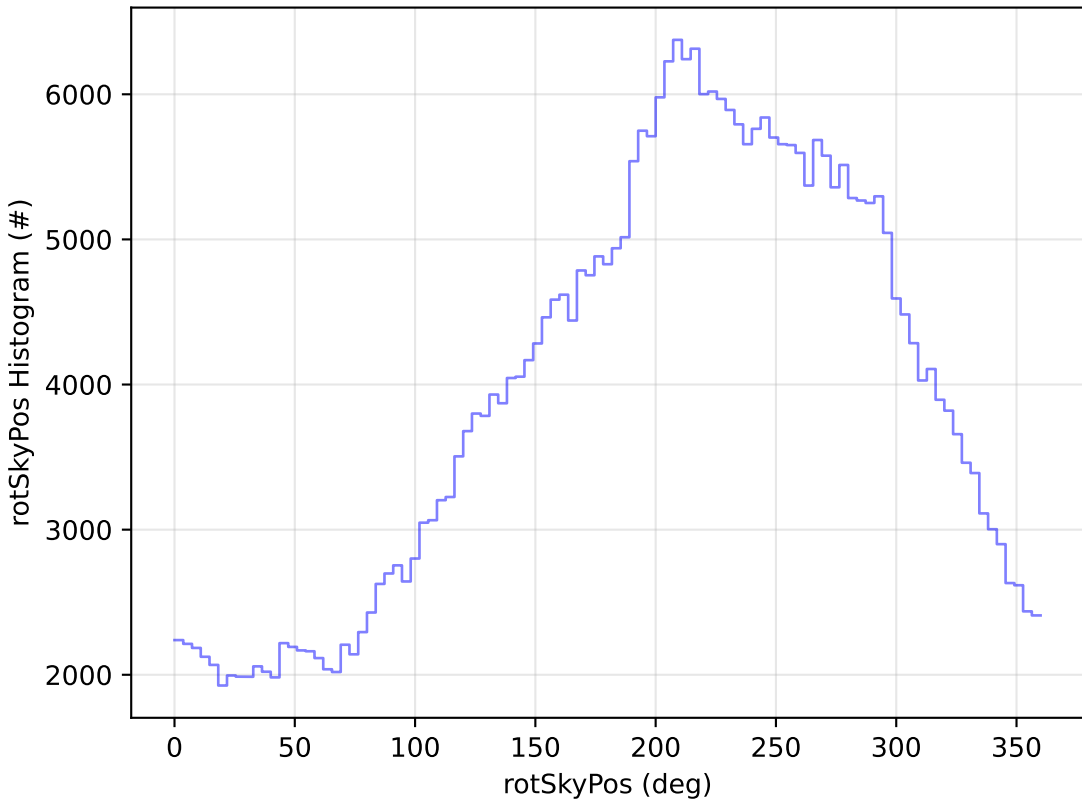
too_elab_r8_d2_giz_v3.4_10yrs All sky y band: rotSkyPos Histogram
