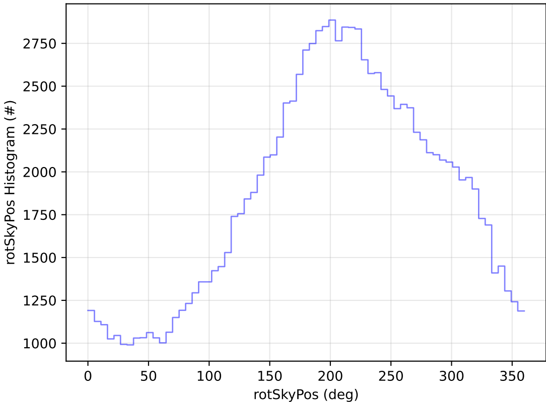
too_elab_r8_d2_giz_v3.4_10yrs All sky u band: rotSkyPos Histogram
