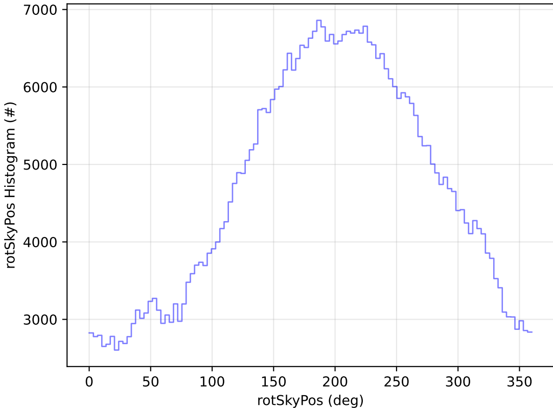
too_elab_r8_d2_giz_v3.4_10yrs All sky r band: rotSkyPos Histogram
