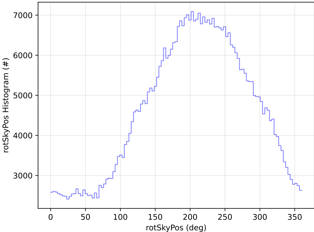
too_elab_r8_d2_giz_v3.4_10yrs All sky i band: rotSkyPos Histogram
