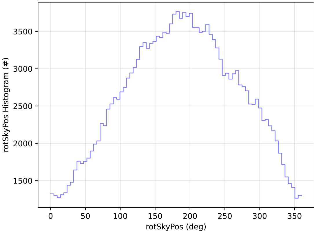
too_elab_r8_d2_giz_v3.4_10yrs All sky g band: rotSkyPos Histogram
