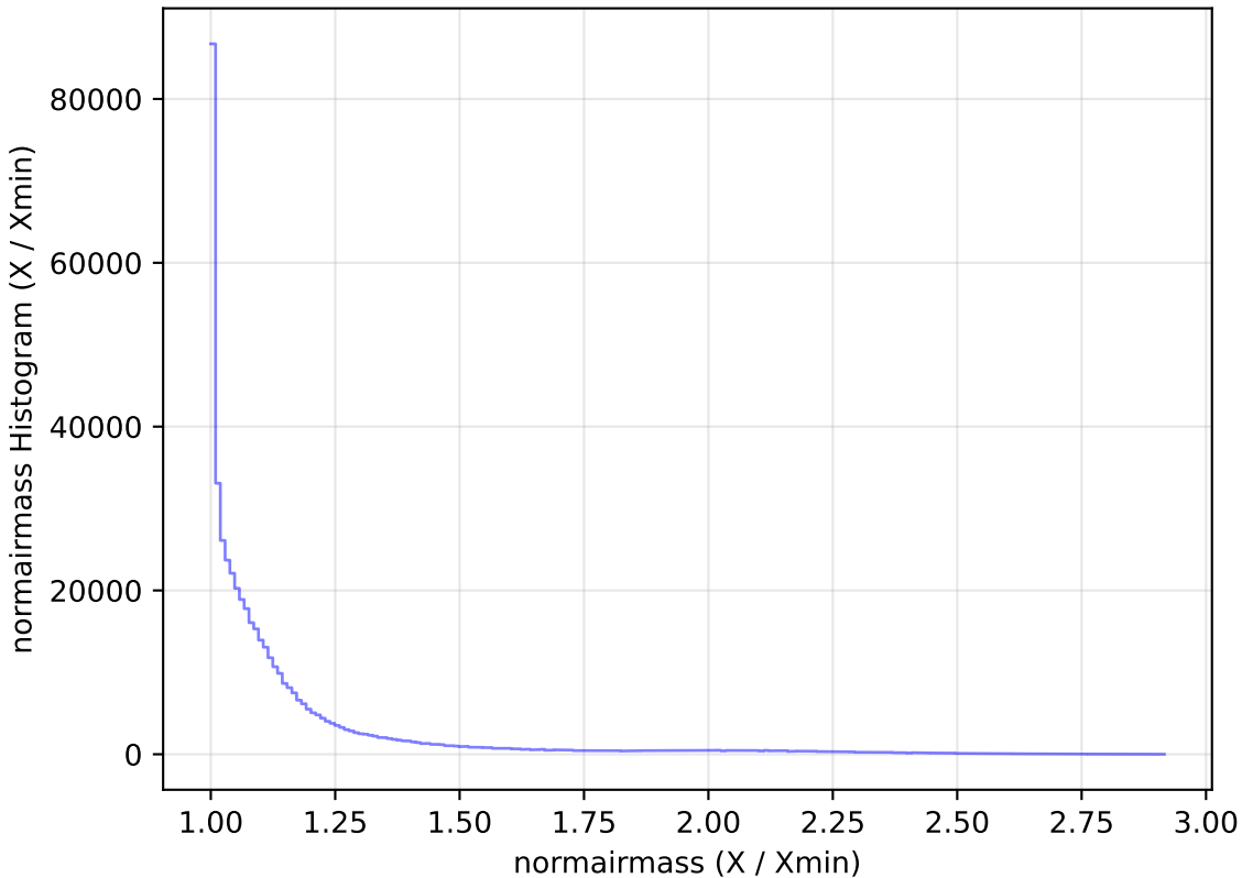
too_elab_r8_d2_giz_v3.4_10yrs WFD i band: normairmass Histogram
