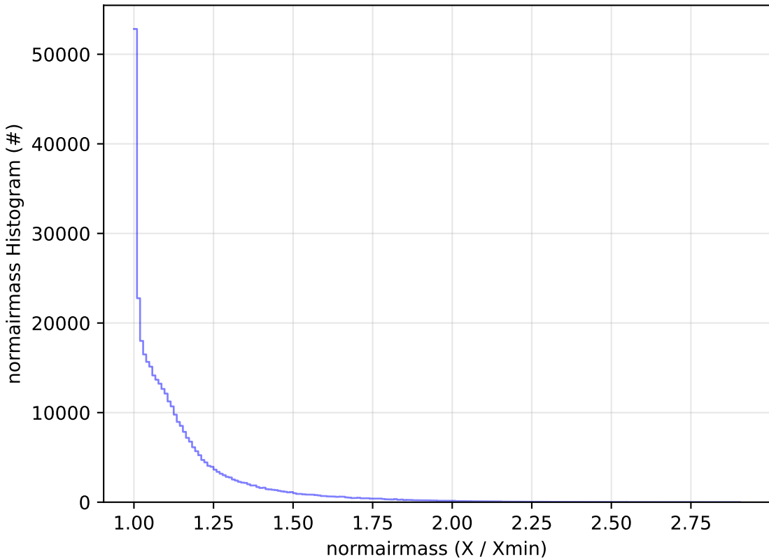
too_elab_r8_d2_giz_v3.4_10yrs All sky y band: normairmass Histogram
