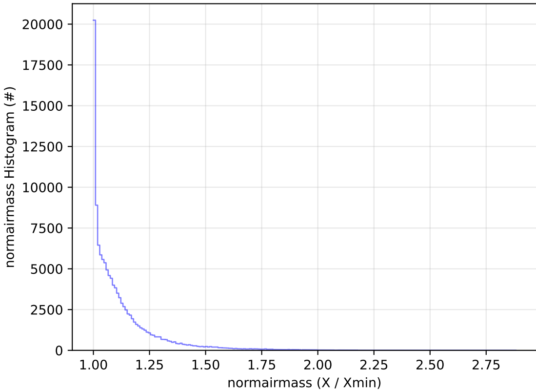
too_elab_r8_d2_giz_v3.4_10yrs All sky u band: normairmass Histogram
