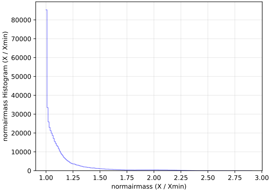
too_elab_r8_d2_giz_v3.4_10yrs All sky r band: normairmass Histogram
