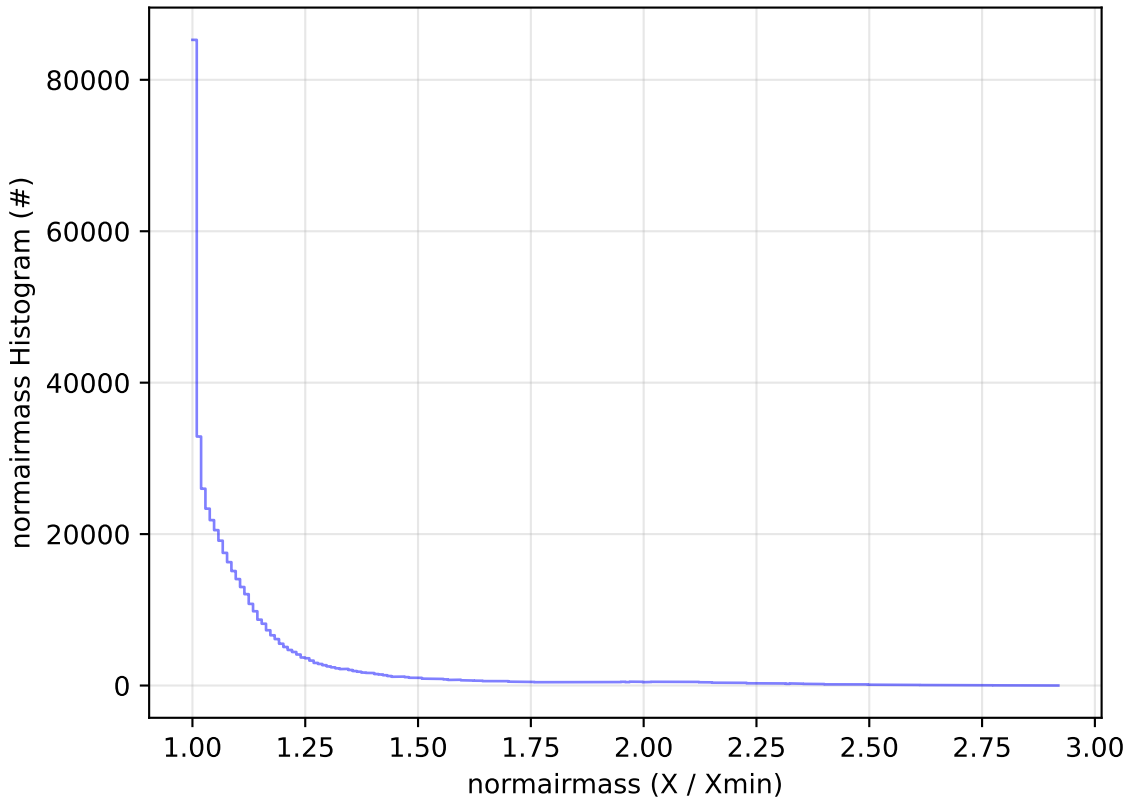
too_elab_r8_d2_giz_v3.4_10yrs All sky i band: normairmass Histogram
