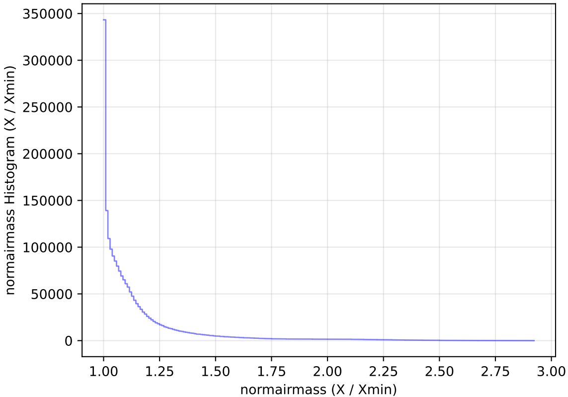
too_elab_r8_d2_giz_v3.4_10yrs All sky all bands: normairmass Histogram
