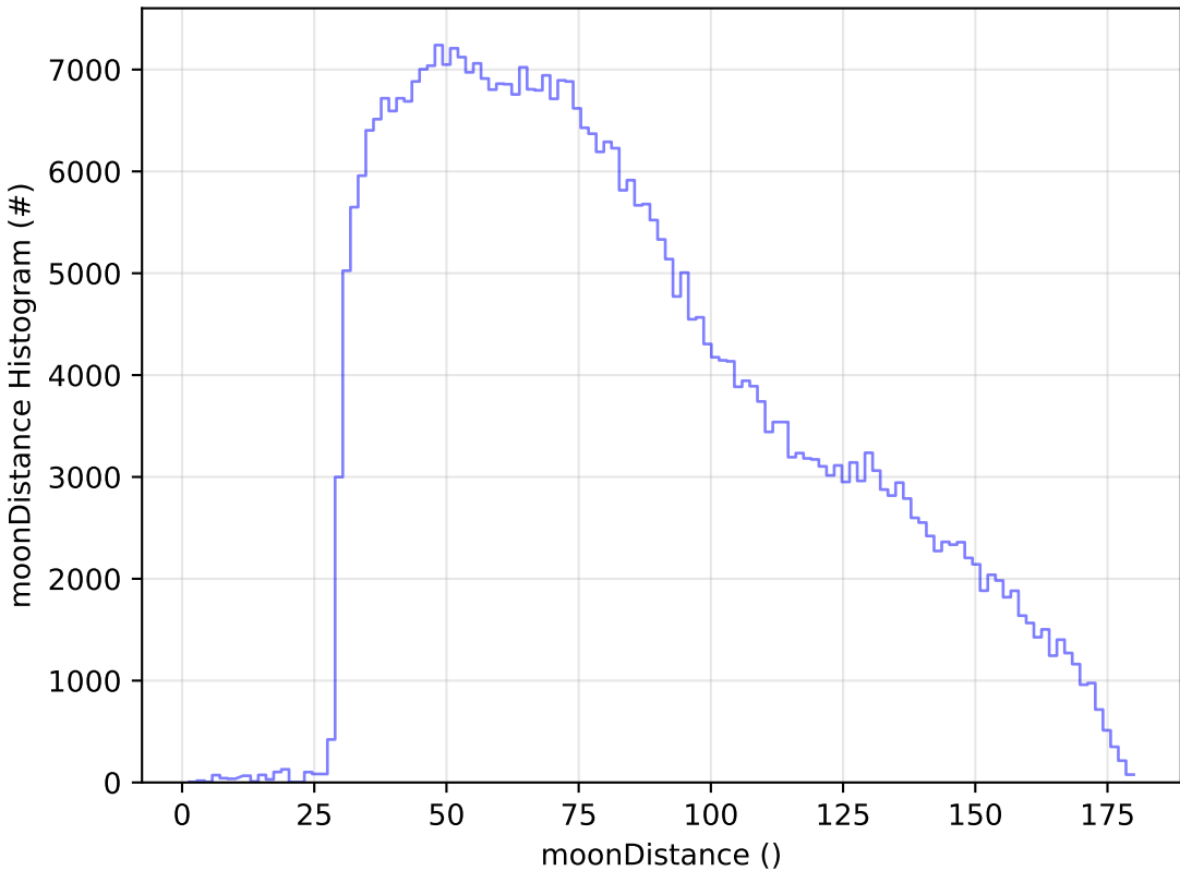
too_elab_r8_d2_giz_v3.4_10yrs WFD z band: moonDistance Histogram
