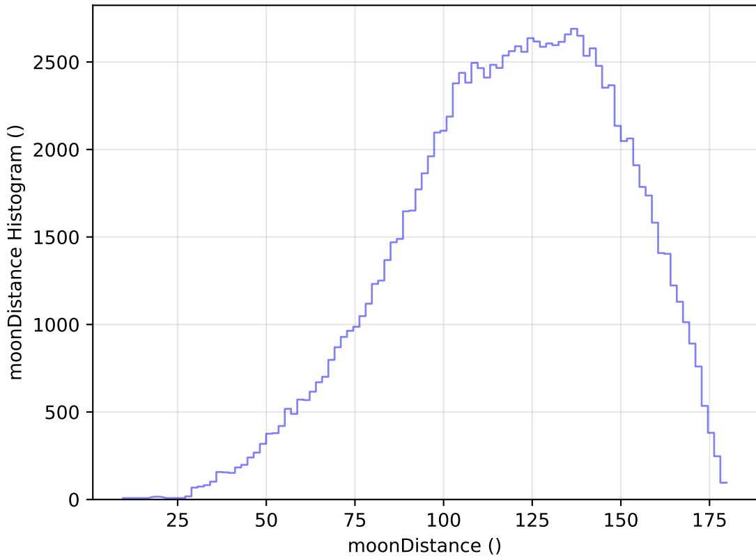
too_elab_r8_d2_giz_v3.4_10yrs WFD u band: moonDistance Histogram
