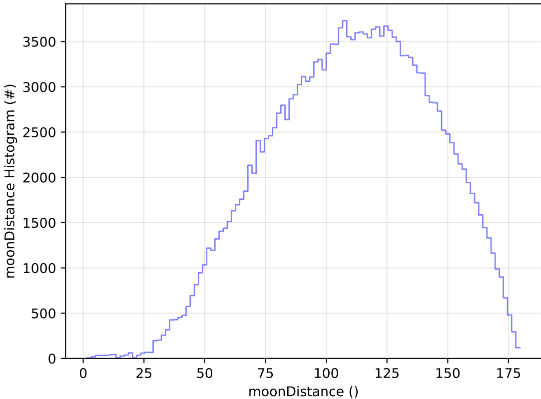
too_elab_r8_d2_giz_v3.4_10yrs WFD g band: moonDistance Histogram
