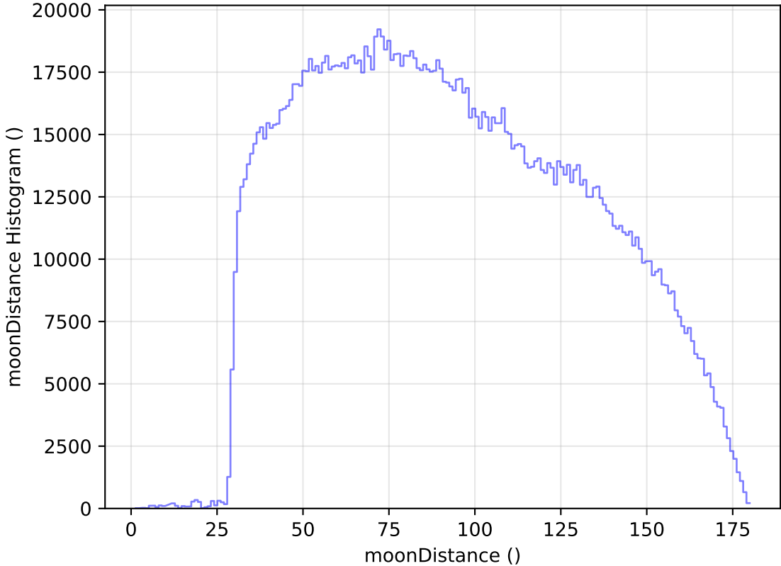
too_elab_r8_d2_giz_v3.4_10yrs WFD all bands: moonDistance Histogram
