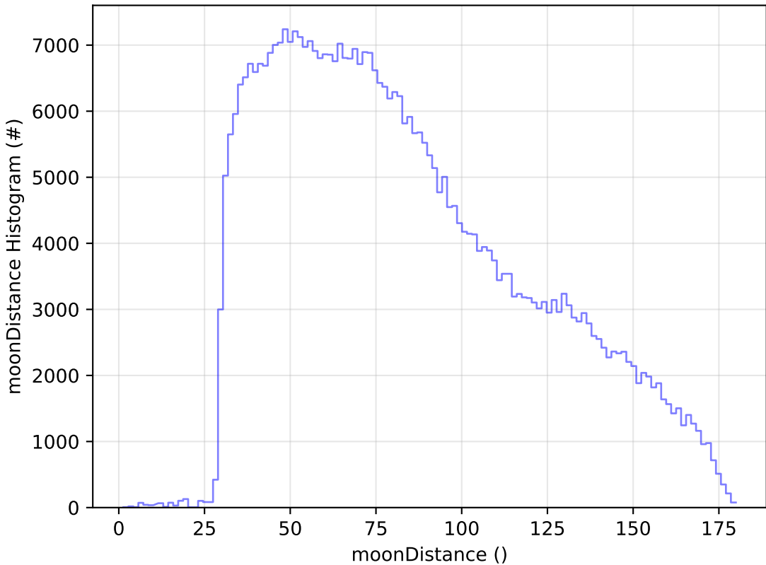
too_elab_r8_d2_giz_v3.4_10yrs All sky z band: moonDistance Histogram
