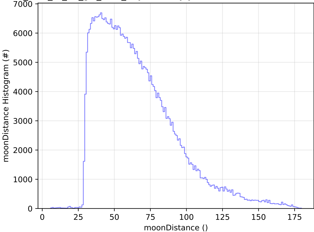
too_elab_r8_d2_giz_v3.4_10yrs All sky y band: moonDistance Histogram
