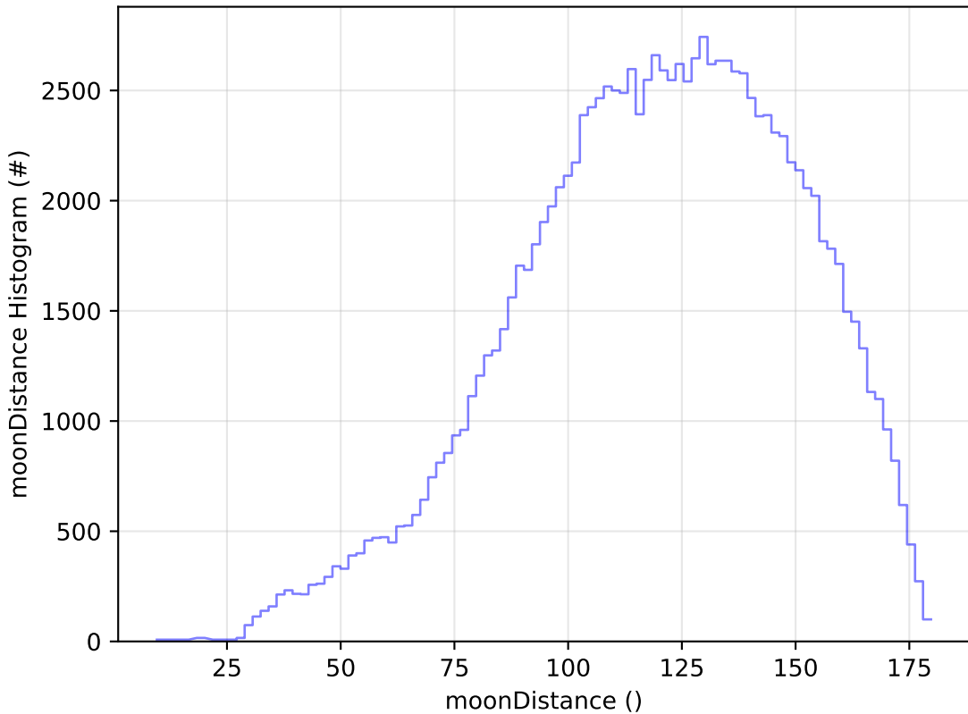
too_elab_r8_d2_giz_v3.4_10yrs All sky u band: moonDistance Histogram
