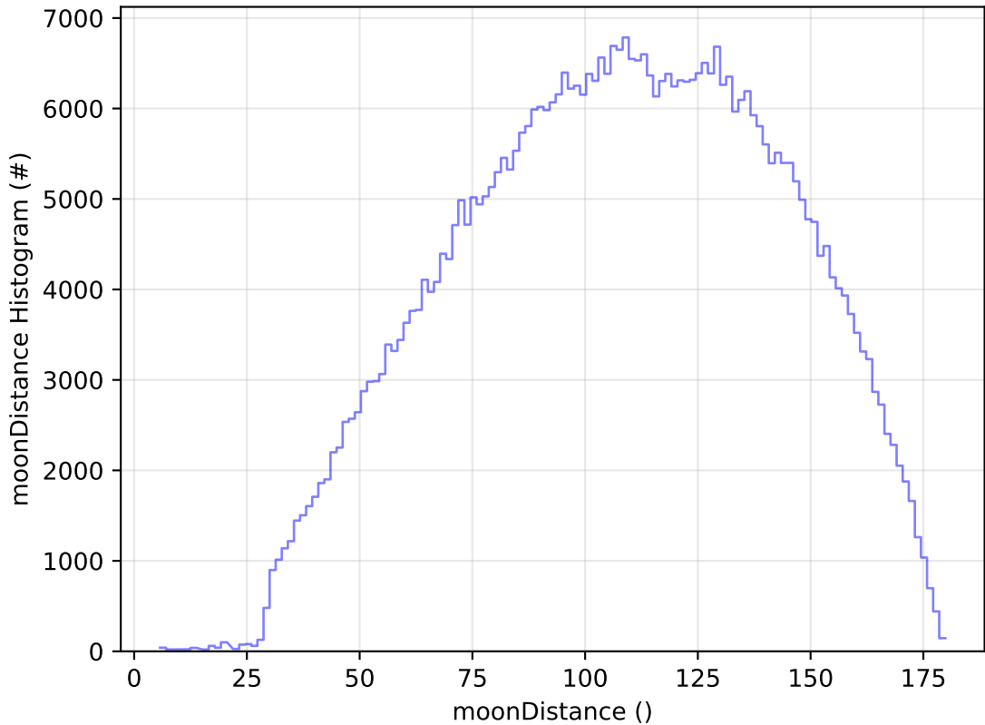
too_elab_r8_d2_giz_v3.4_10yrs All sky r band: moonDistance Histogram
