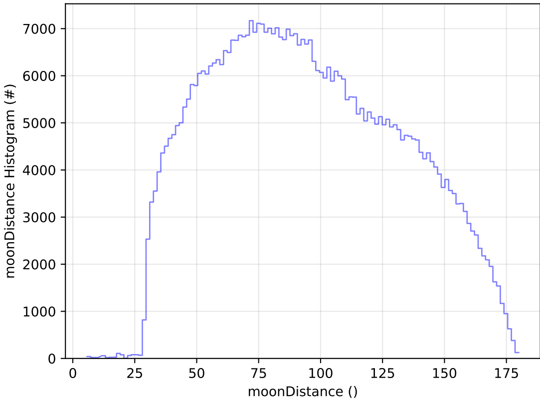
too_elab_r8_d2_giz_v3.4_10yrs All sky i band: moonDistance Histogram
