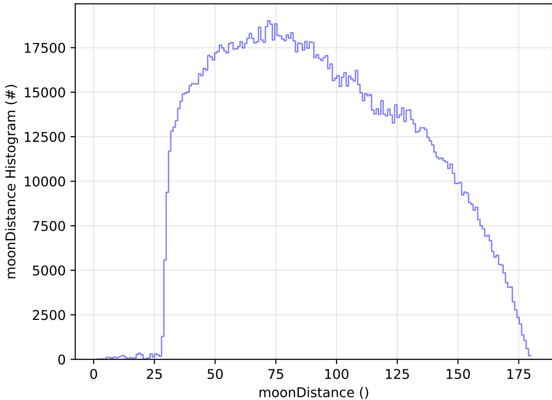
too_elab_r8_d2_giz_v3.4_10yrs All sky all bands: moonDistance Histogram
