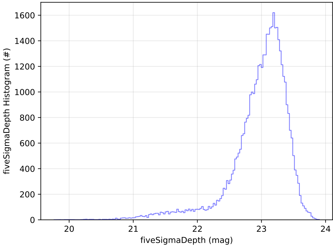
too_elab_r8_d2_giz_v3.4_10yrs Yr 1 z band: fiveSigmaDepth Histogram
