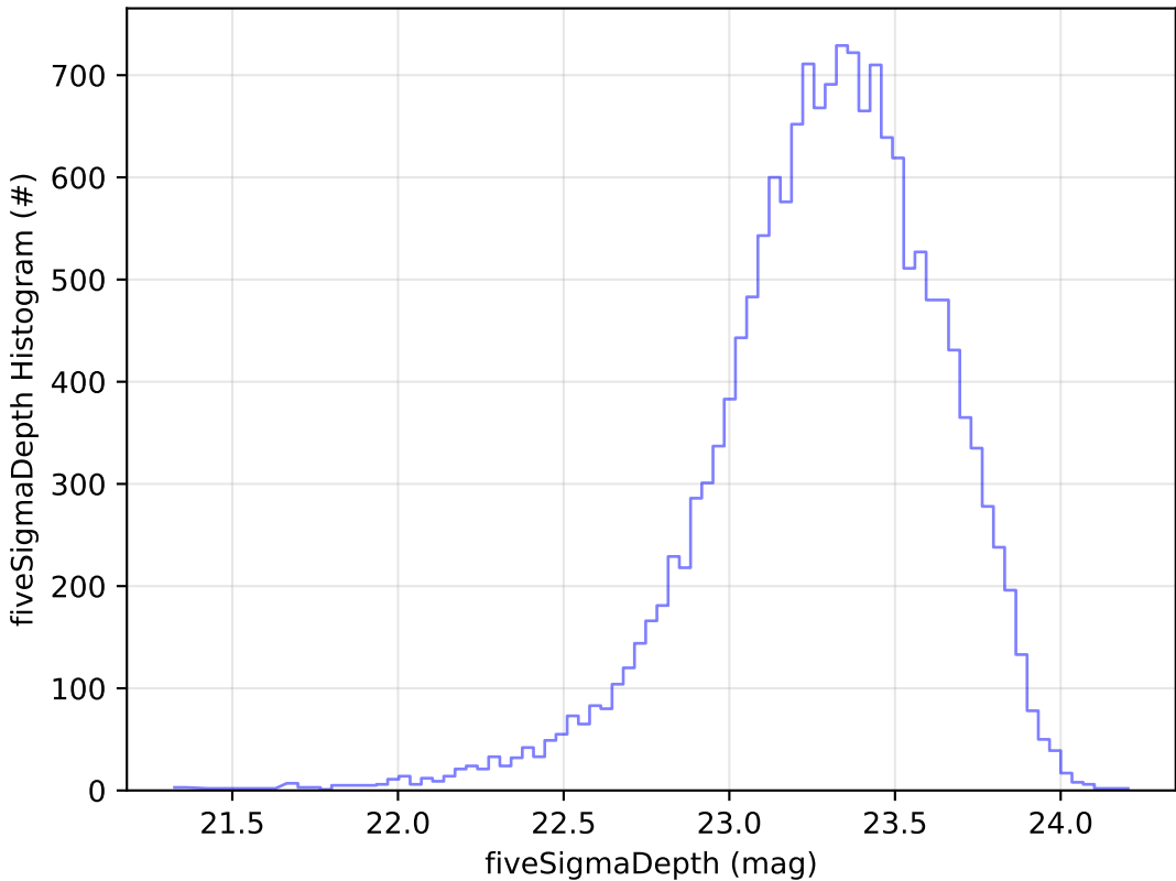
too_elab_r8_d2_giz_v3.4_10yrs Yr 1 u band: fiveSigmaDepth Histogram
