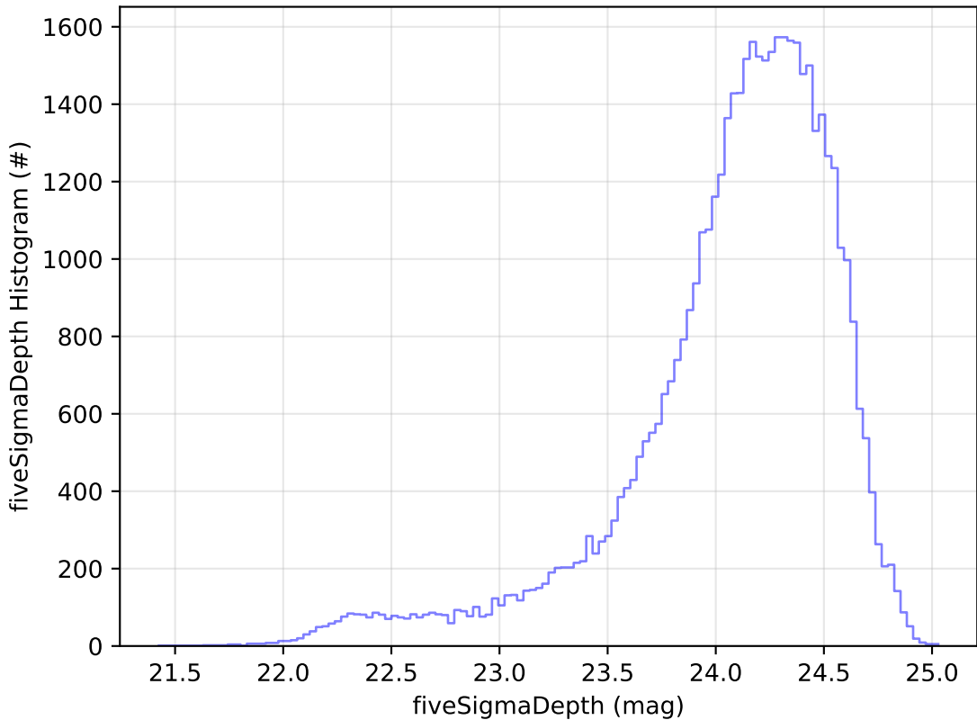
too_elab_r8_d2_giz_v3.4_10yrs Yr 1 r band: fiveSigmaDepth Histogram
