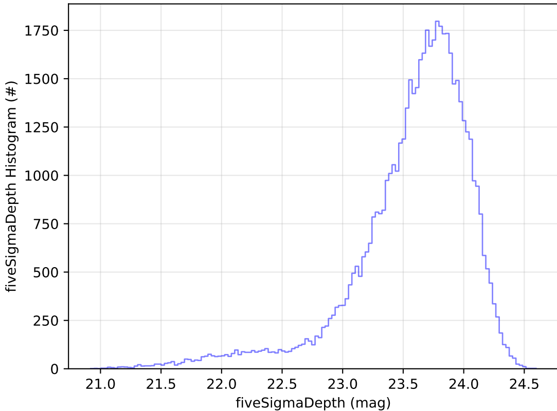
too_elab_r8_d2_giz_v3.4_10yrs Yr 1 i band: fiveSigmaDepth Histogram
