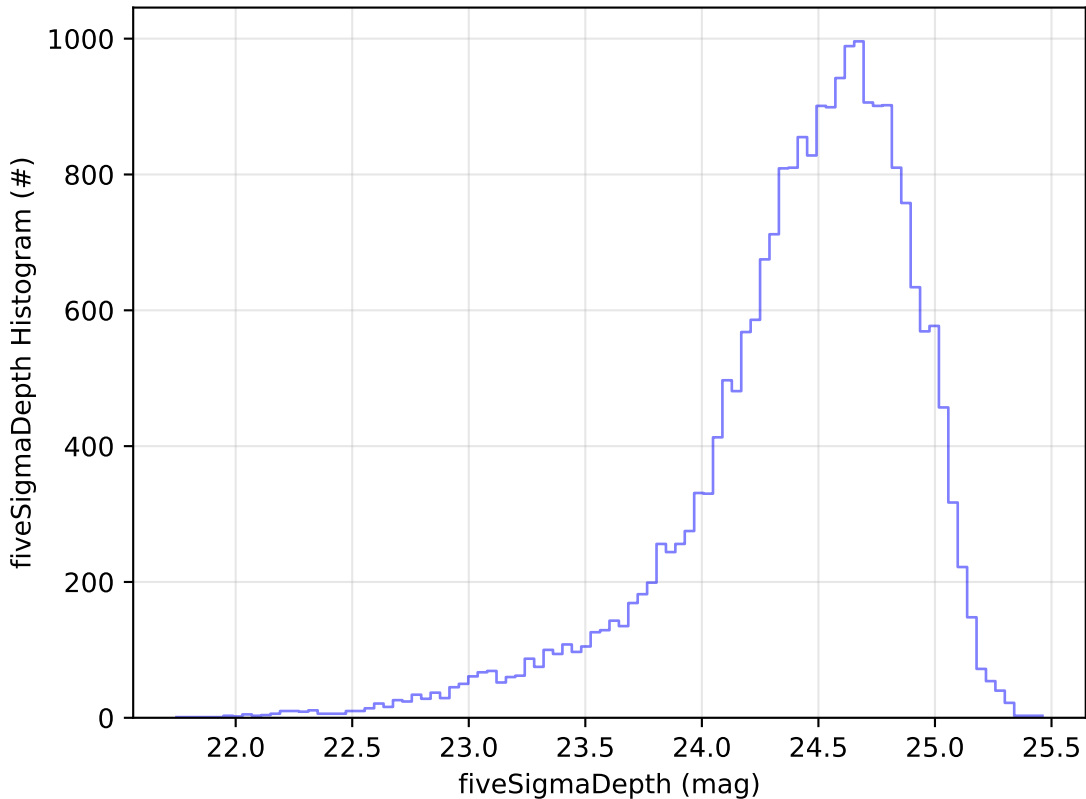
too_elab_r8_d2_giz_v3.4_10yrs Yr 1 g band: fiveSigmaDepth Histogram
