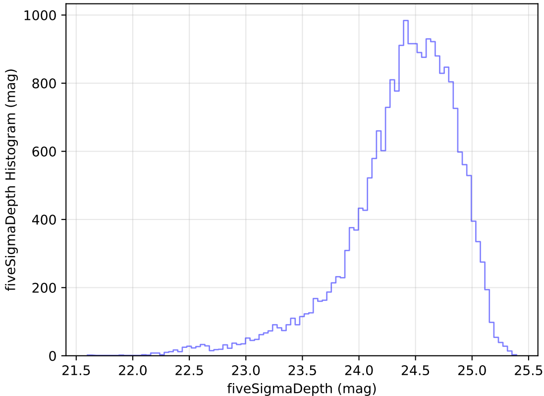
too_elab_r8_d2_giz_v3.4_10yrs Yr 1 g band: fiveSigmaDepth Histogram
