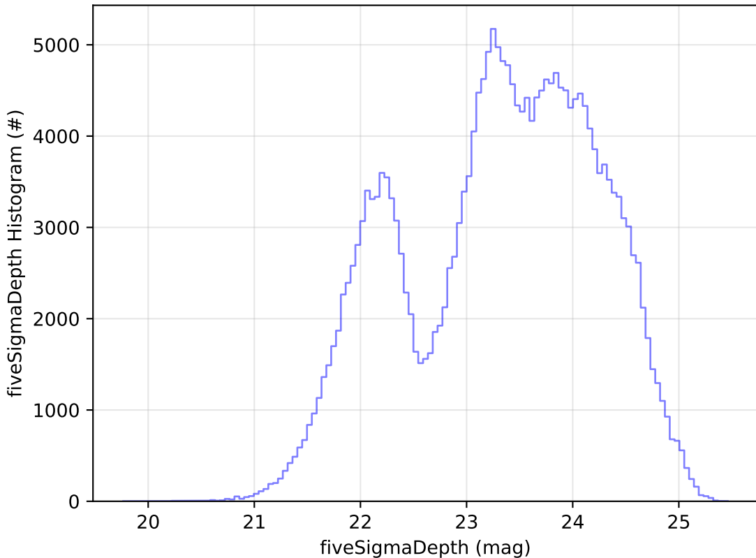
too_elab_r8_d2_giz_v3.4_10yrs Yr 1 all bands: fiveSigmaDepth Histogram
